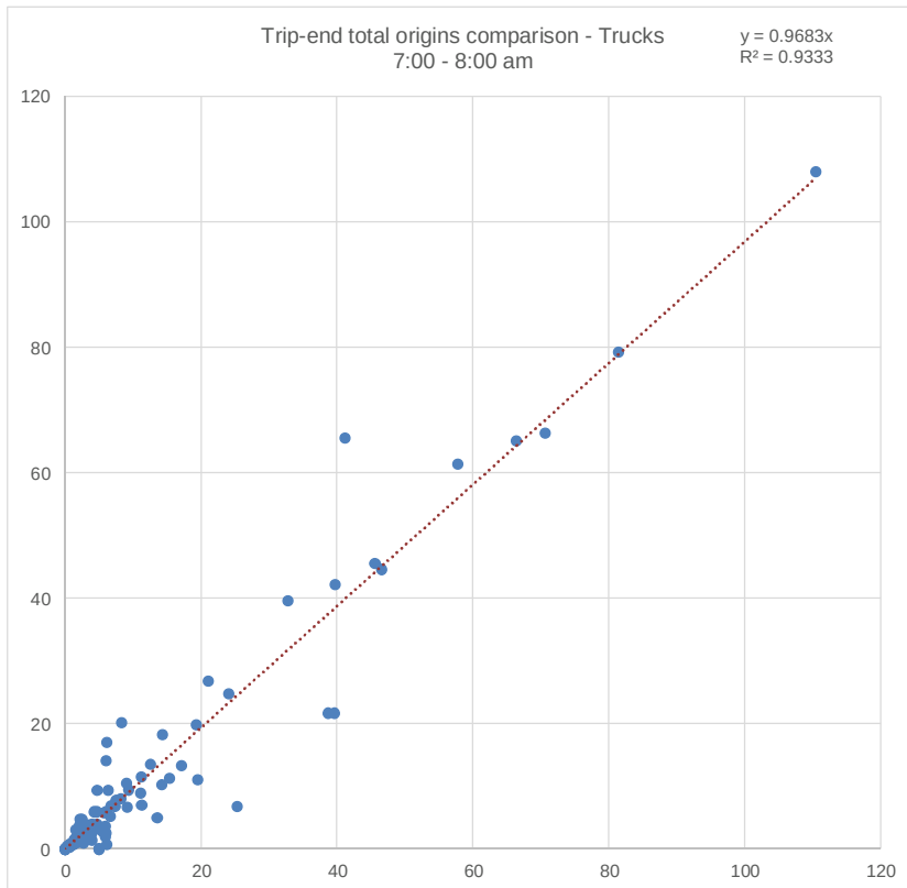
Figure A.11 Trip-ends regression – Trucks – 7.00–8.00 am – Origins
