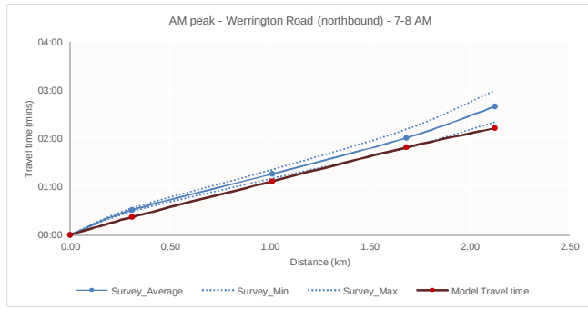
Route 5 – AM peak 7.00–8.00
