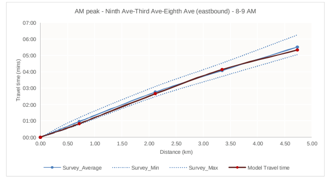
Route 3 – AM peak 8.00–9.00
