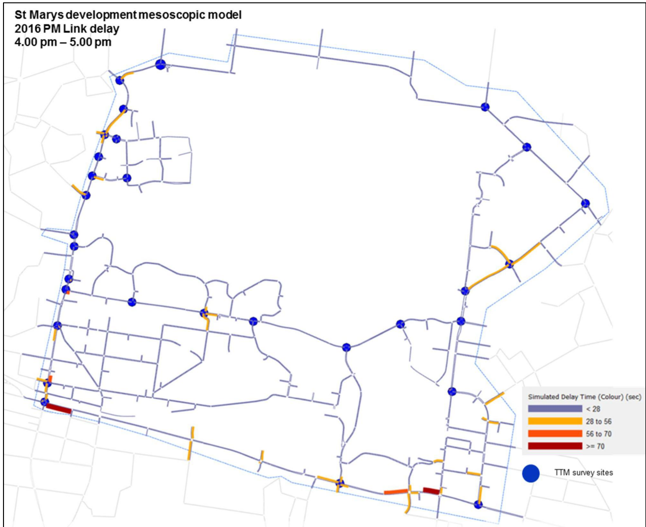
Network delay plot – 4.00 pm to 5.00 pm
