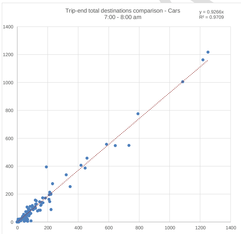
Figure A.10 Trip-ends regression – Cars – 7.00–8.00 am – Destinations
