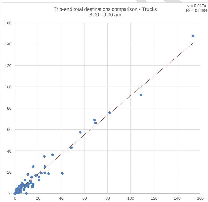
Figure A.16 Trip-ends regression – Trucks – 8.00–9.00 am – Destinations
