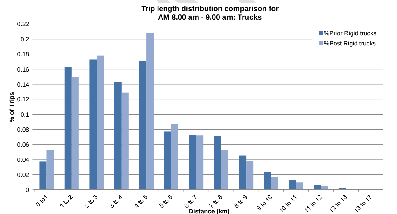
Figure A.6 Trip length distribution –Trucks – 8.00–9.00 am
