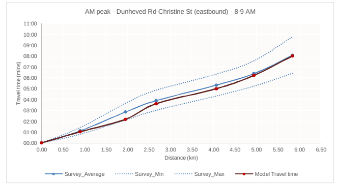
Route 4 – AM peak 8.00–9.00
