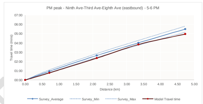
Route 3 – PM peak 5.00–6.00
