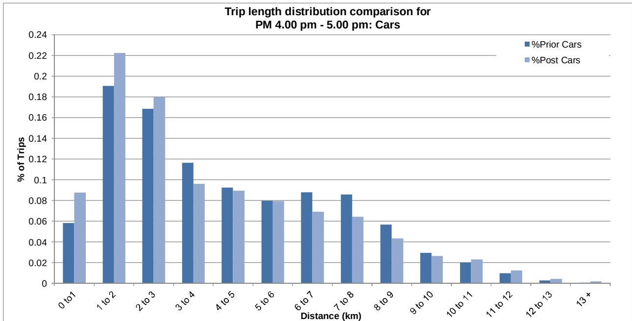
Figure A.3 Trip length distribution – Cars – 4.00–5.00 pm
