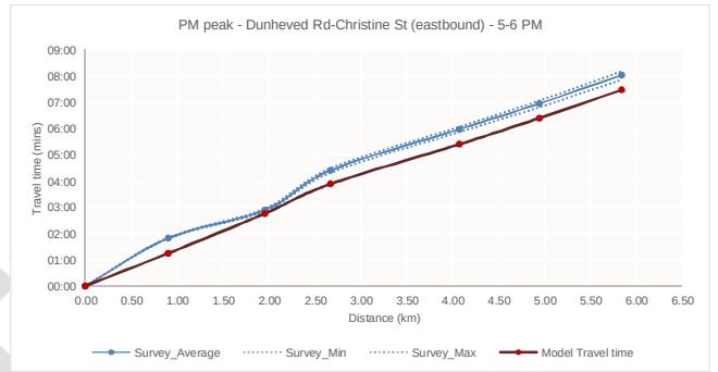
Route 4 – PM peak 5.00–6.00
