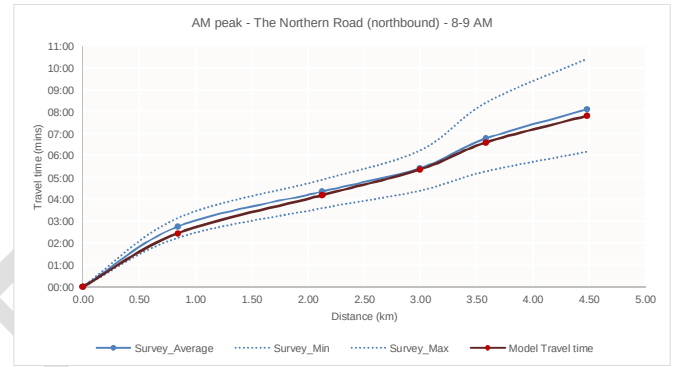
Route 1 – AM peak 8.00–9.00
