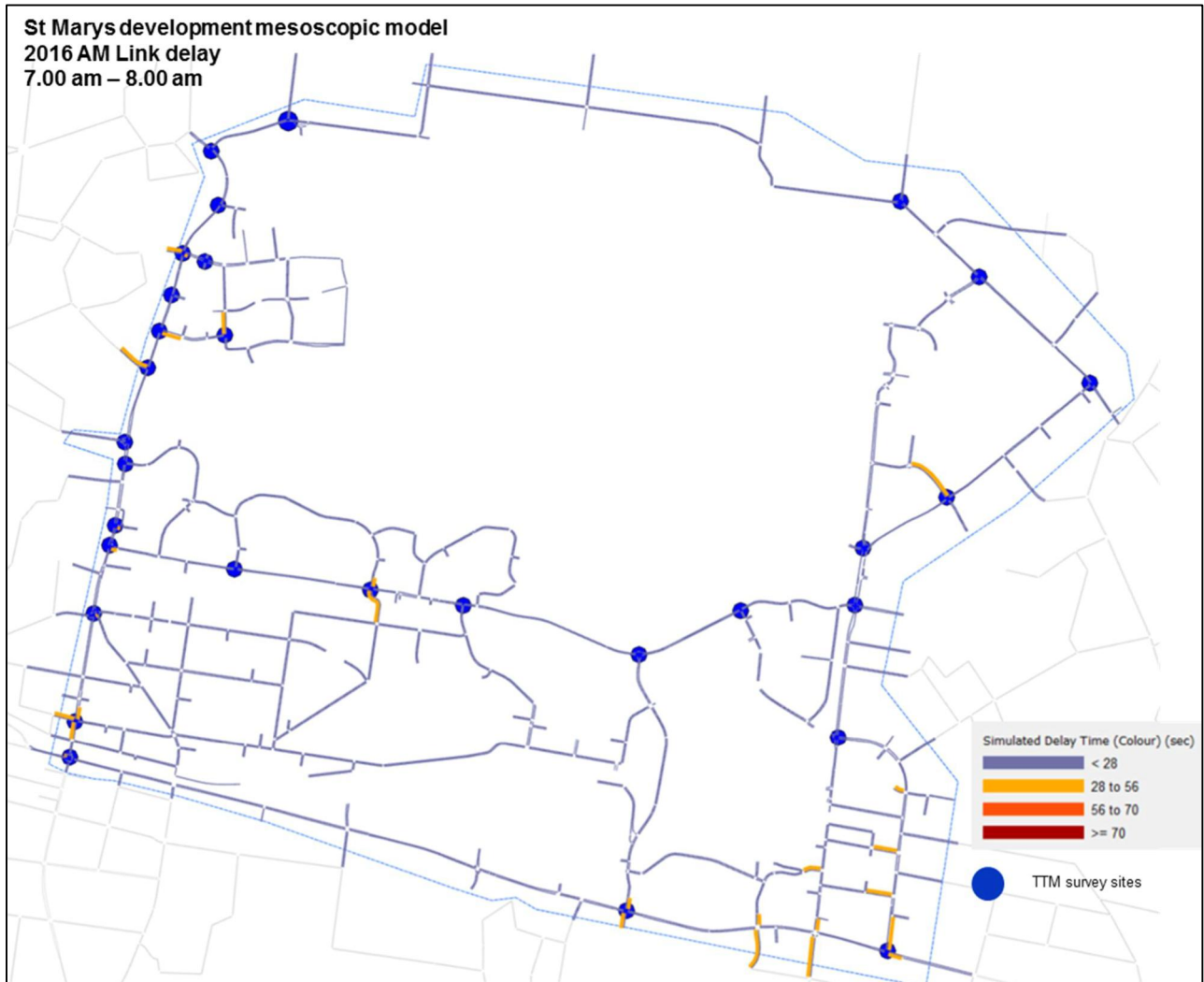
Network delay plot – 7.00 am to 8.00 am
