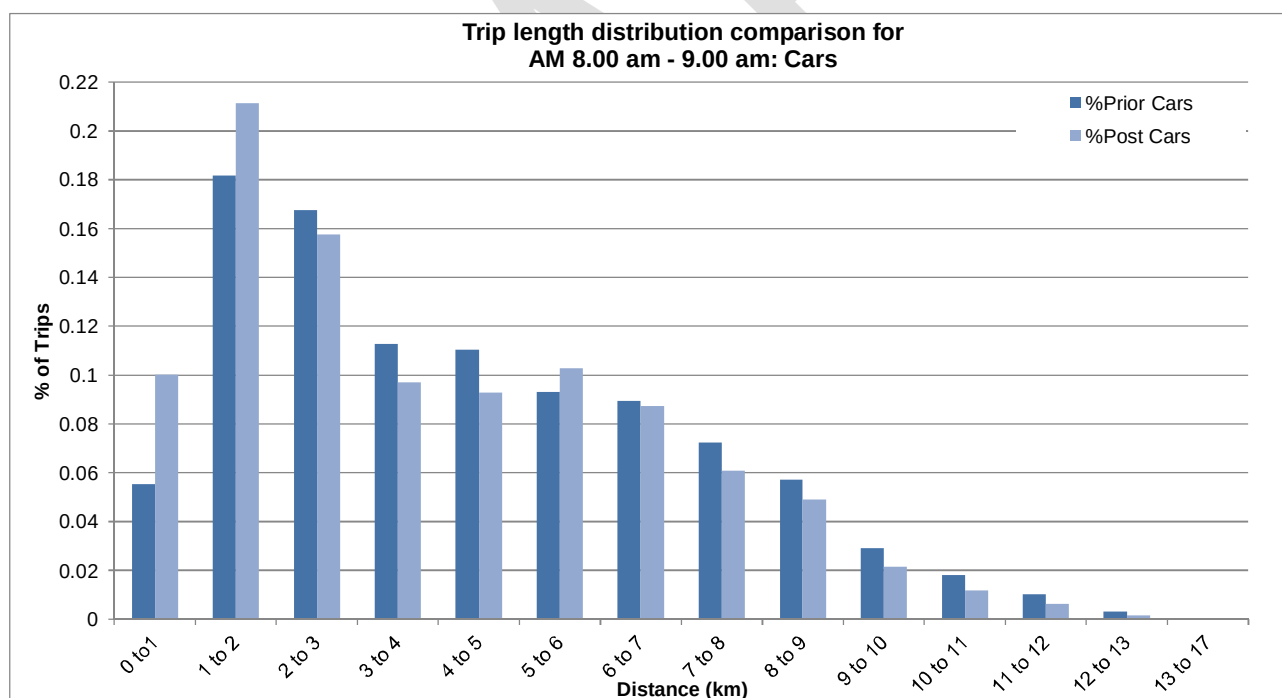
Figure A.2 Trip length distribution – Cars – 8.00–9.00 am
