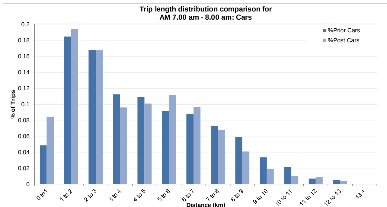
Figure A.1 Trip length distribution – Cars – 7.00–8.00 am
