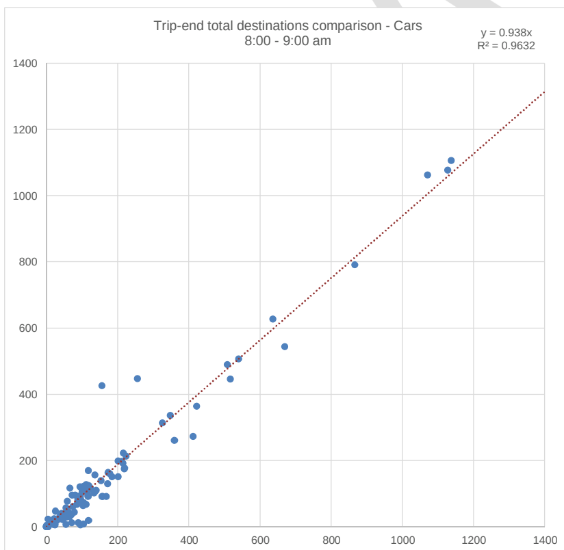
Figure A.14 Trip-ends regression – Cars – 8.00–9.00 am – Destinations
