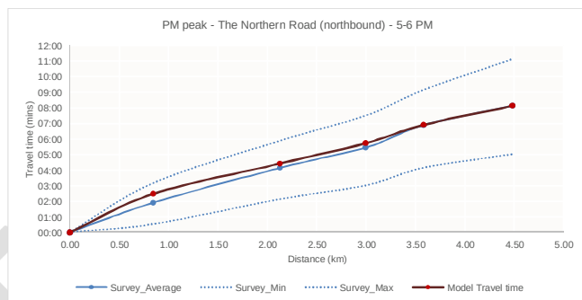
Route 1 – PM peak 5.00–6.00
