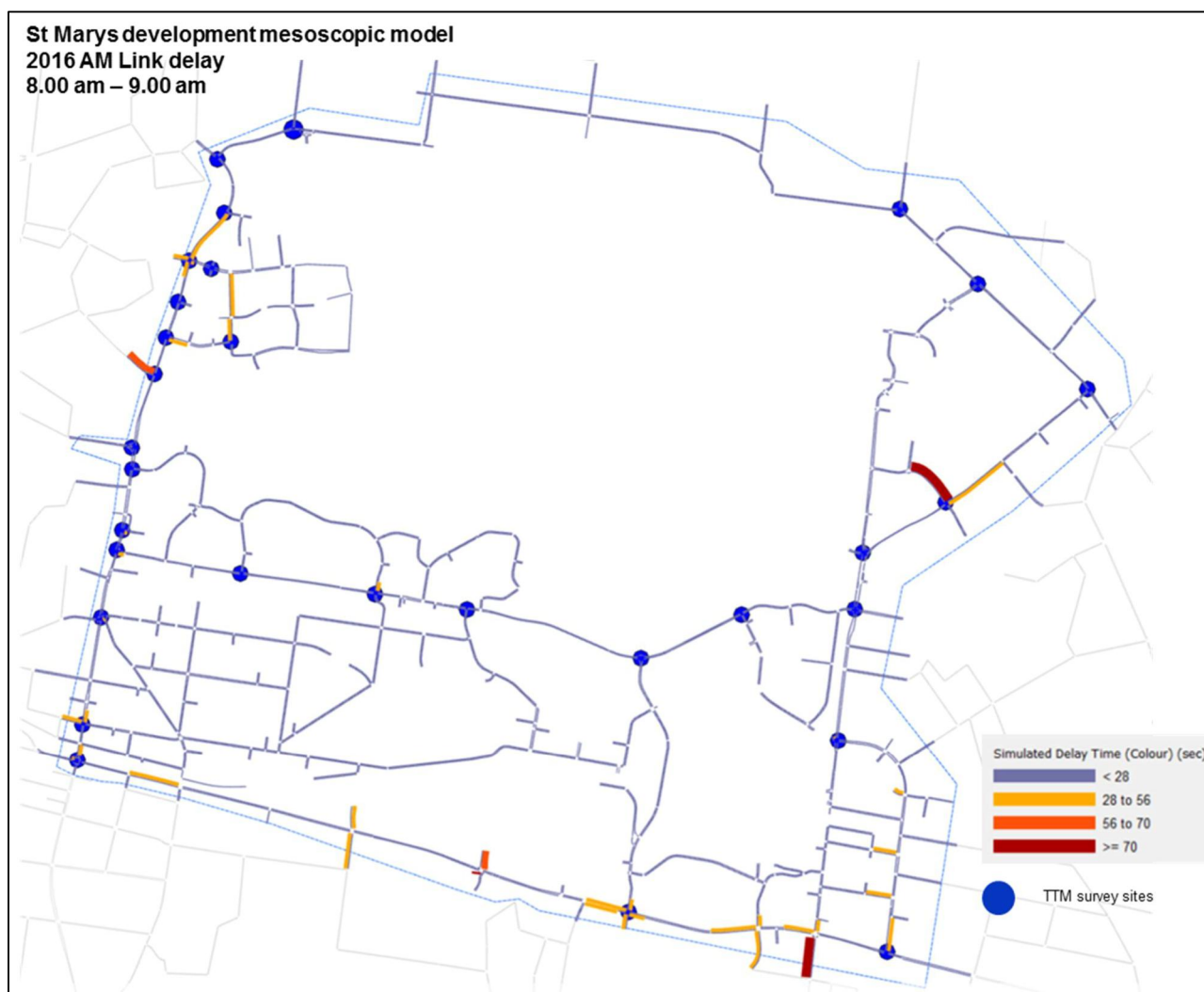
Network delay plot – 8.00 am to 9.00 am
