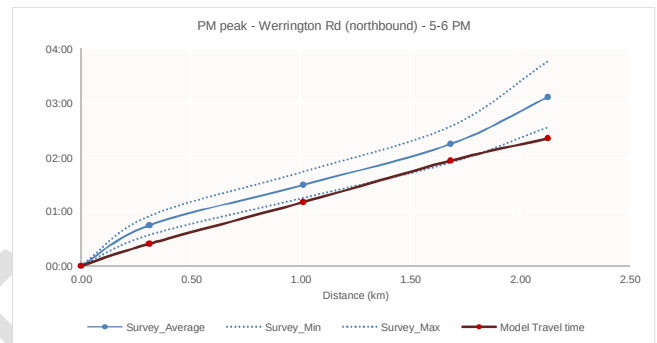
Route 5 – PM peak 5.00–6.00
