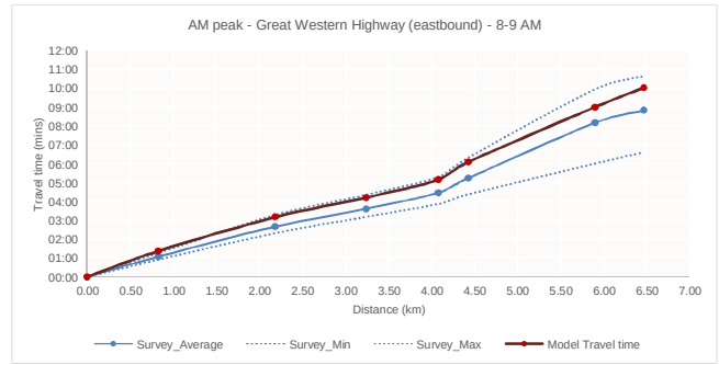
Route 6 – AM peak 8.00–9.00
