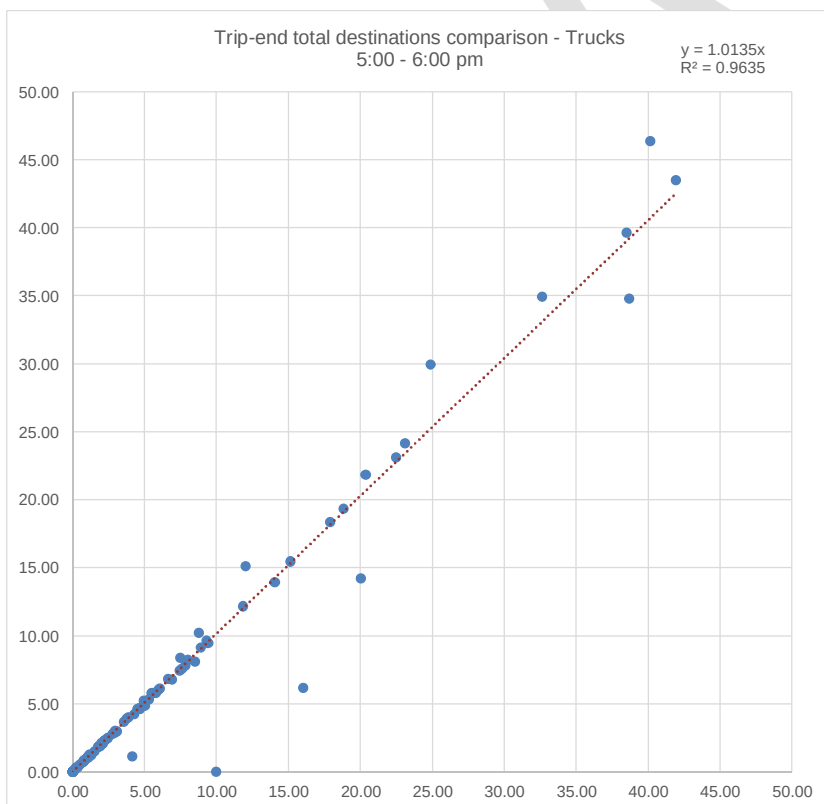
Figure A.24 Trip-ends regression –Trucks – 5.00–6.00 pm – Destinations
