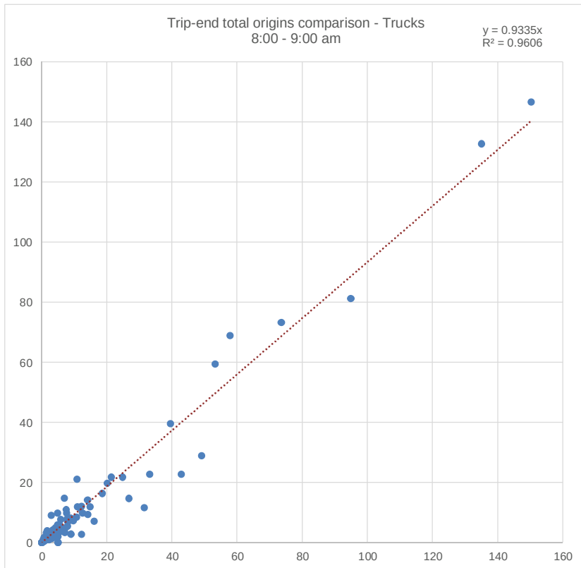
Figure A.15 Trip-ends regression – Trucks – 8.00–9.00 am – Origins
