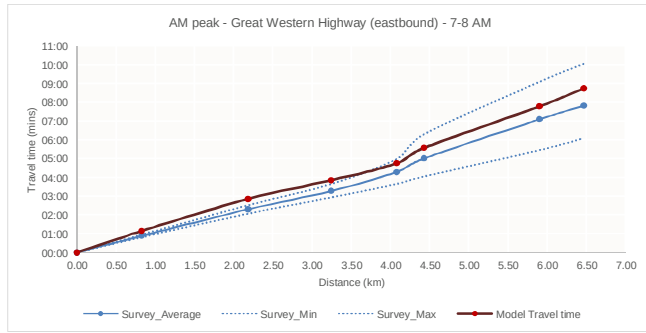
Route 6 – AM peak 7.00–8.00
