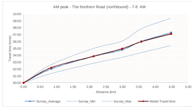
Route 1 – AM peak 7.00–8.00
