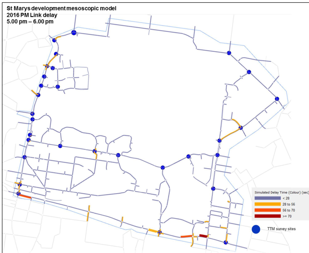
Network delay plot – 5.00 pm to 6.00 pm
