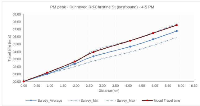
Route 4 – PM peak 4.00–5.00
