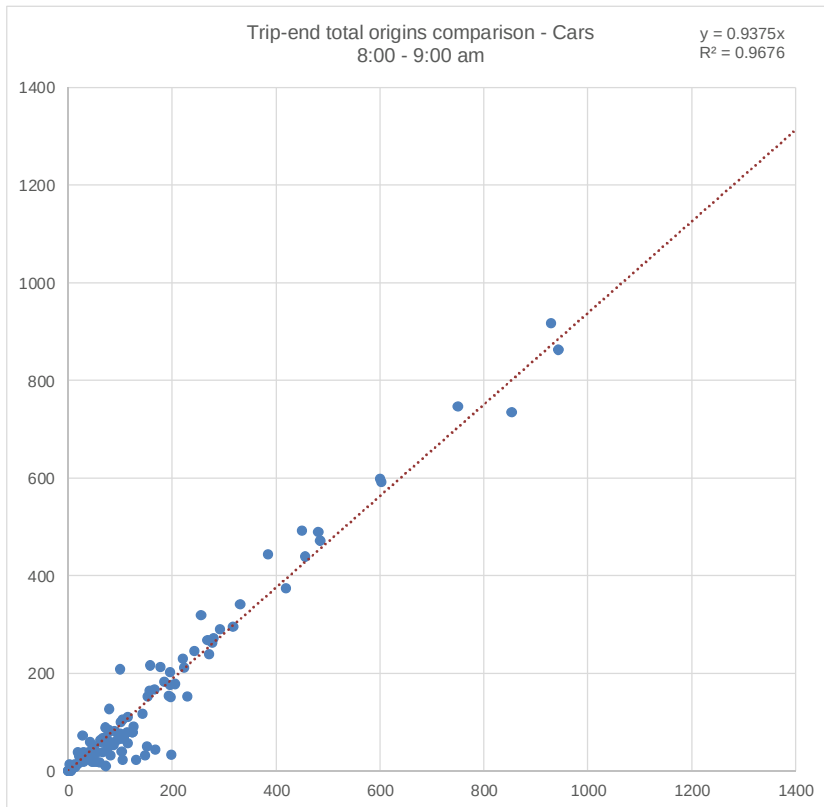
Figure A.13 Trip-ends regression – Cars – 8.00–9.00 am – Origins
