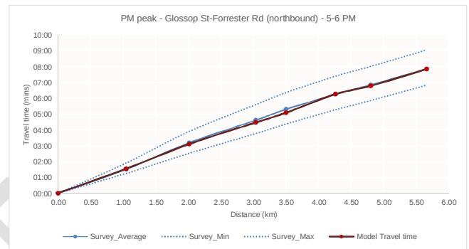
Route 2 – PM peak 5.00–6.00
