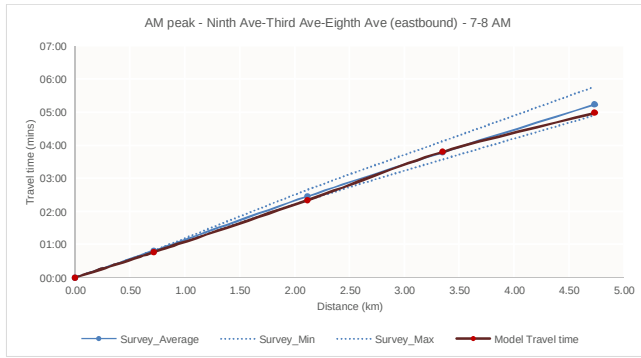
Route 3 – AM peak 7.00–8.00
