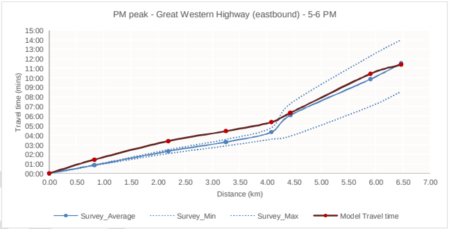
Route 6 – PM peak 5.00–6.00
