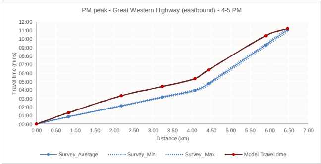
Route 6 – PM peak 4.00–5.00
