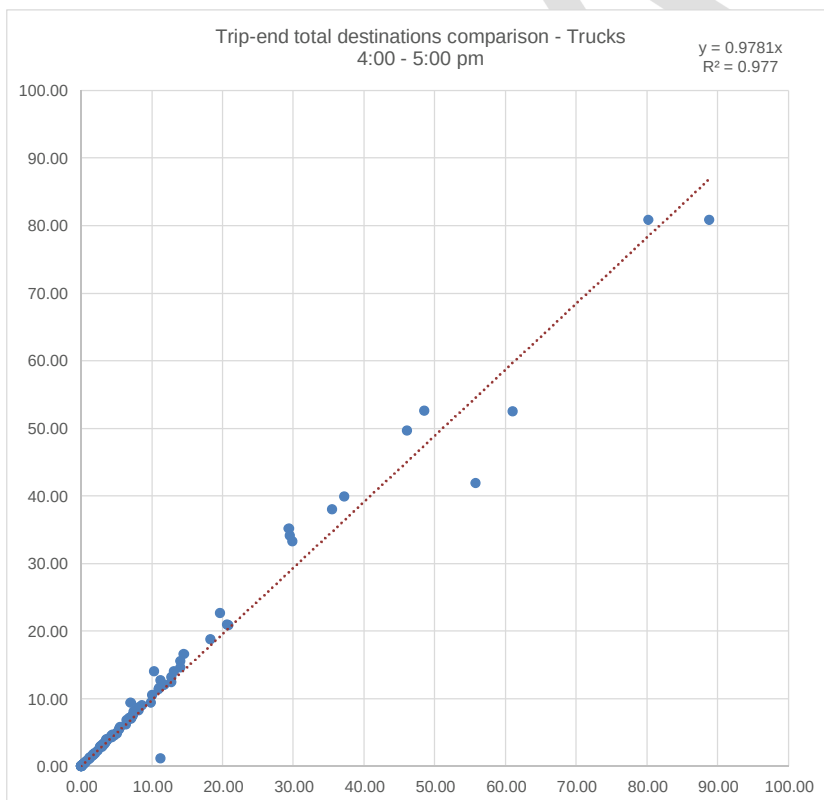
Figure A.20 Trip-ends regression –Trucks – 4.00–5.00 pm – Destinations
