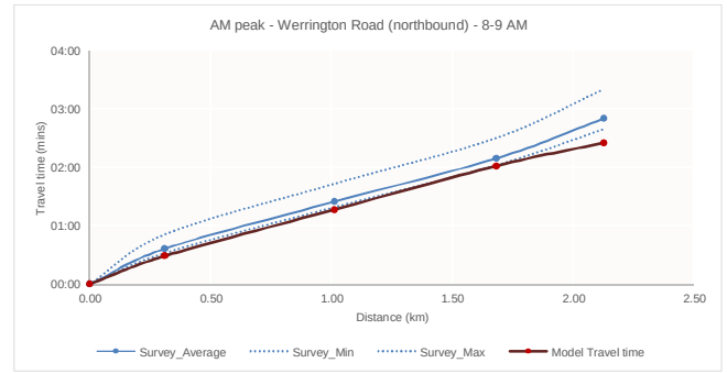
Route 5 – AM peak 8.00–9.00
