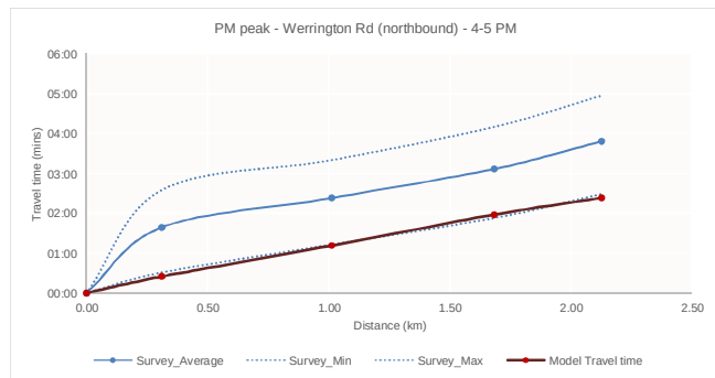
Route 5 – PM peak 4.00–5.00
