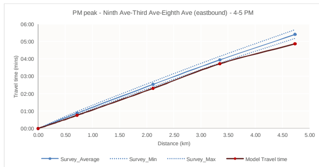
Route 3 – PM peak 4.00–5.00
