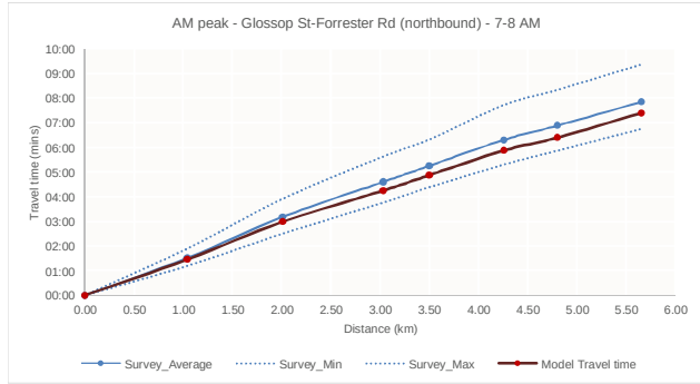
Route 2 – AM peak 7.00–8.00
