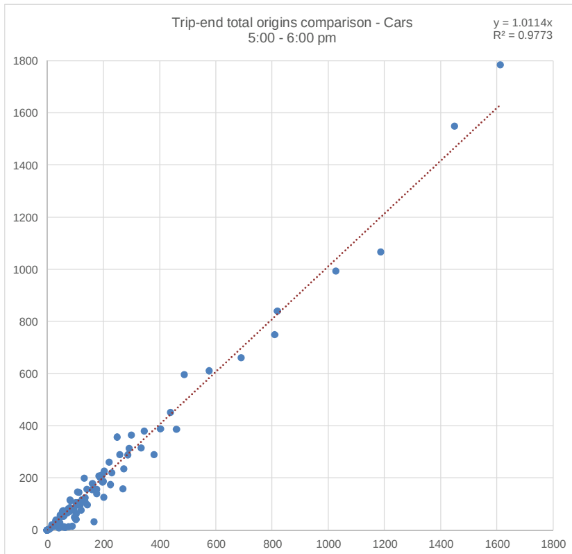
Figure A.21 Trip-ends regression –Cars – 5.00–6.00 pm – Origins
