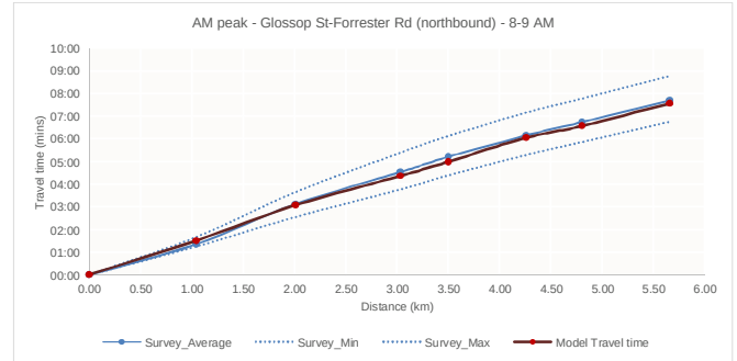
Route 2 – AM peak 8.00–9.00
