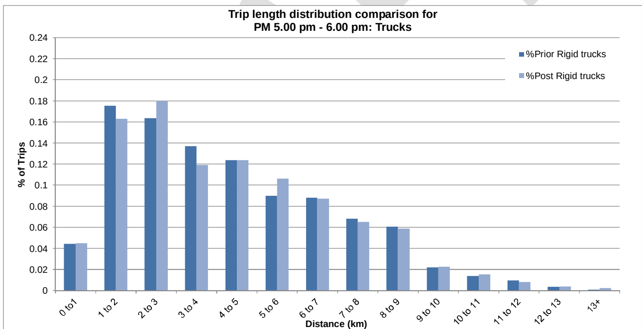
Figure A.8 Trip length distribution –Trucks – 5.00–6.00 pm
