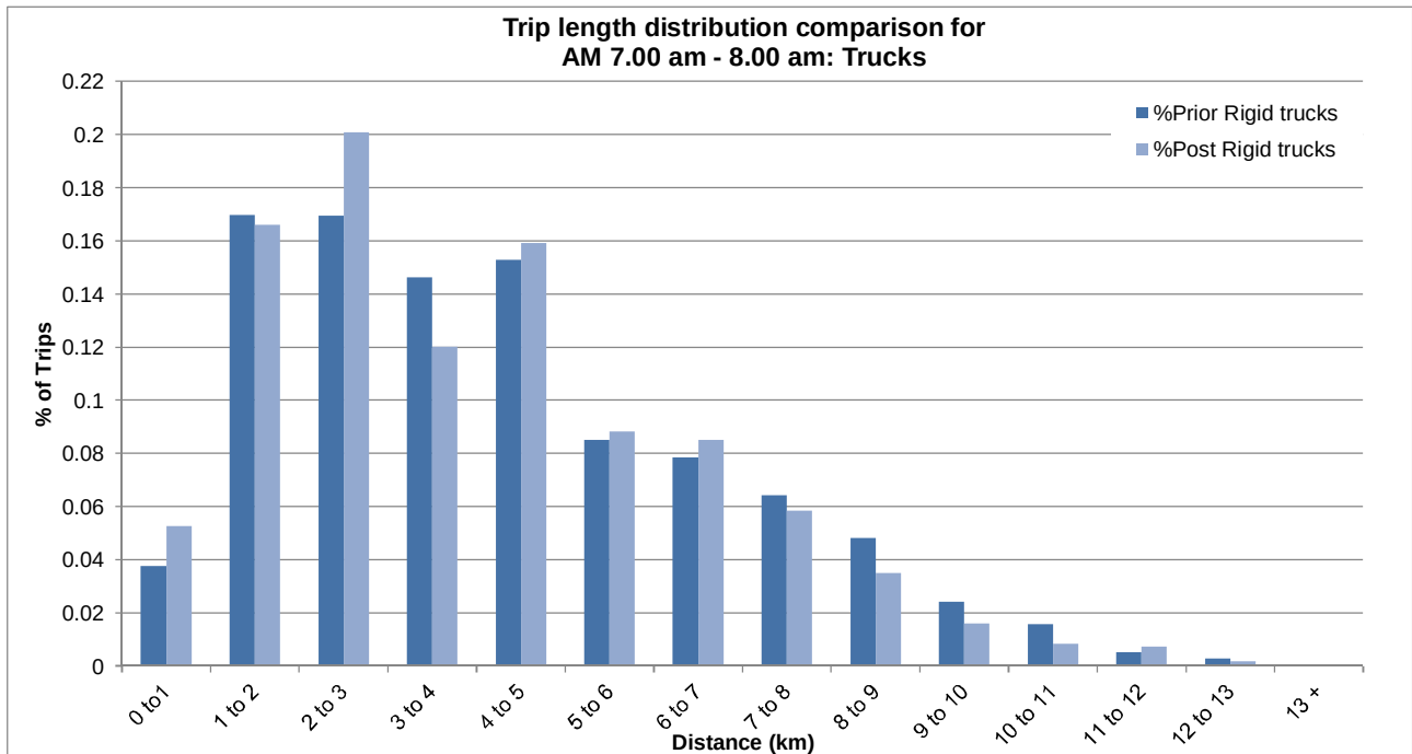
Figure A.5 Trip length distribution –Trucks – 7.00-8.00 am
