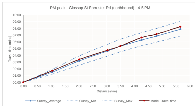
Route 2 – PM peak 4.00–5.00
