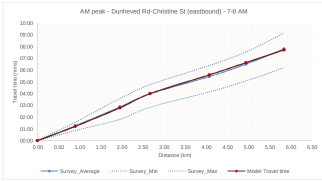
Route 4 – AM peak 7.00–8.00
