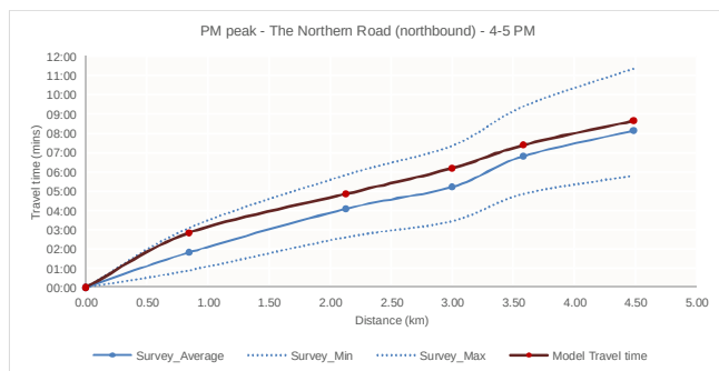
Route 1 – PM peak 4.00–5.00
