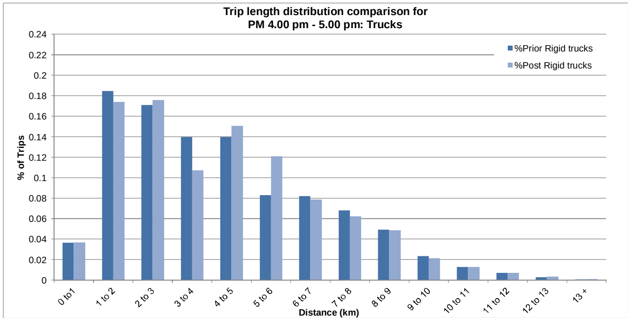
Figure A.7 Trip length distribution –Trucks – 4.00–5.00 pm
