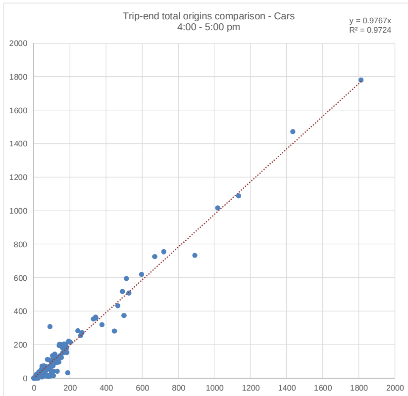
Figure A.17 Trip-ends regression – Cars – 4.00–5.00 pm – Origins
