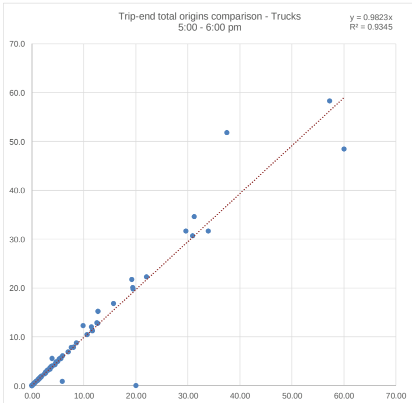
Figure A.23 Trip-ends regression –Trucks – 5.00–6.00 pm – Origins
