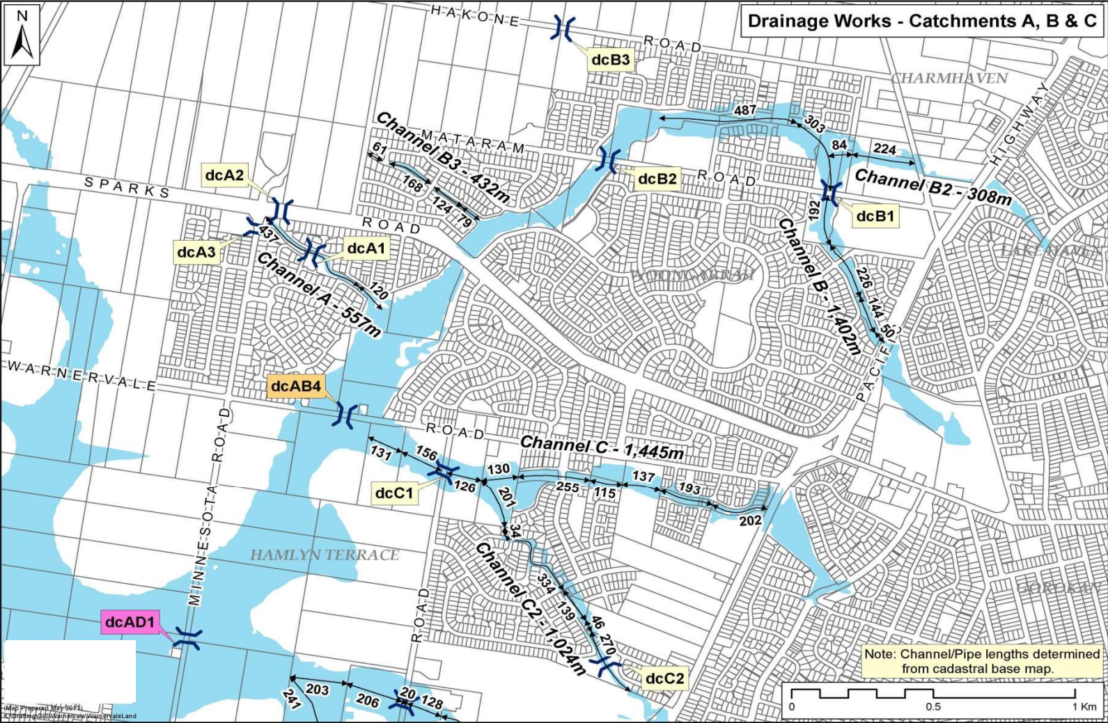
Figure 17 Drainage Works Locations – Catchments A, B & C
