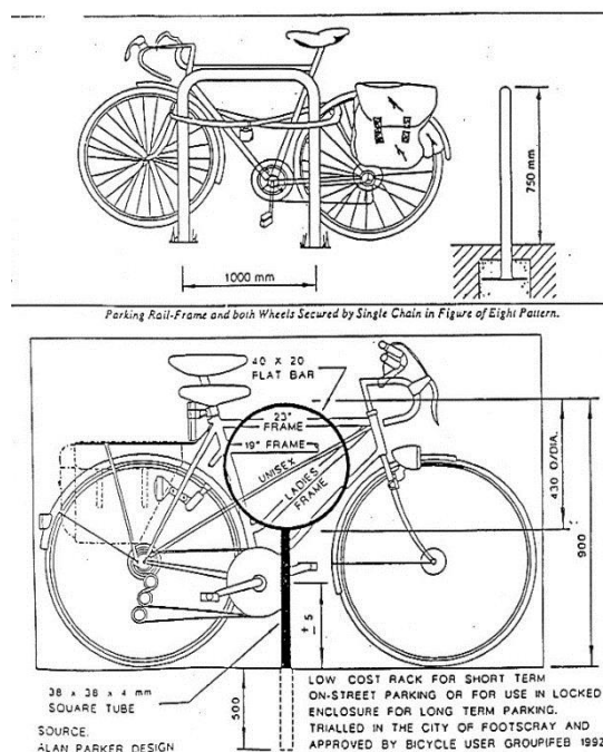
Figure 13 - Bicycle Parking Locking facilities
