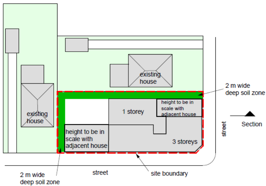
Site Layout
