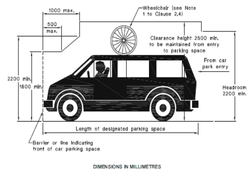
Figure 11 - Vertical Clearance Above Car Spaces for People with Disabilities
