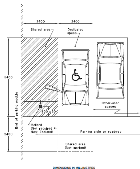
Figure 2B- Parking space dimensions for people with a disability.
