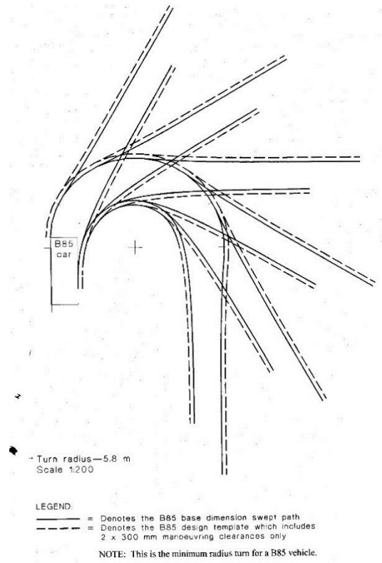
Figure 6 - B85 Car Turning Template - 5.8m Radius
