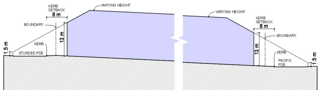
Section C-C
